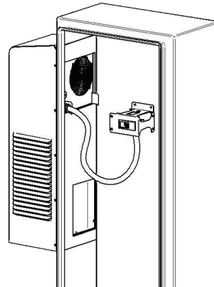
Pictured is the application and installation of the remote controller option
