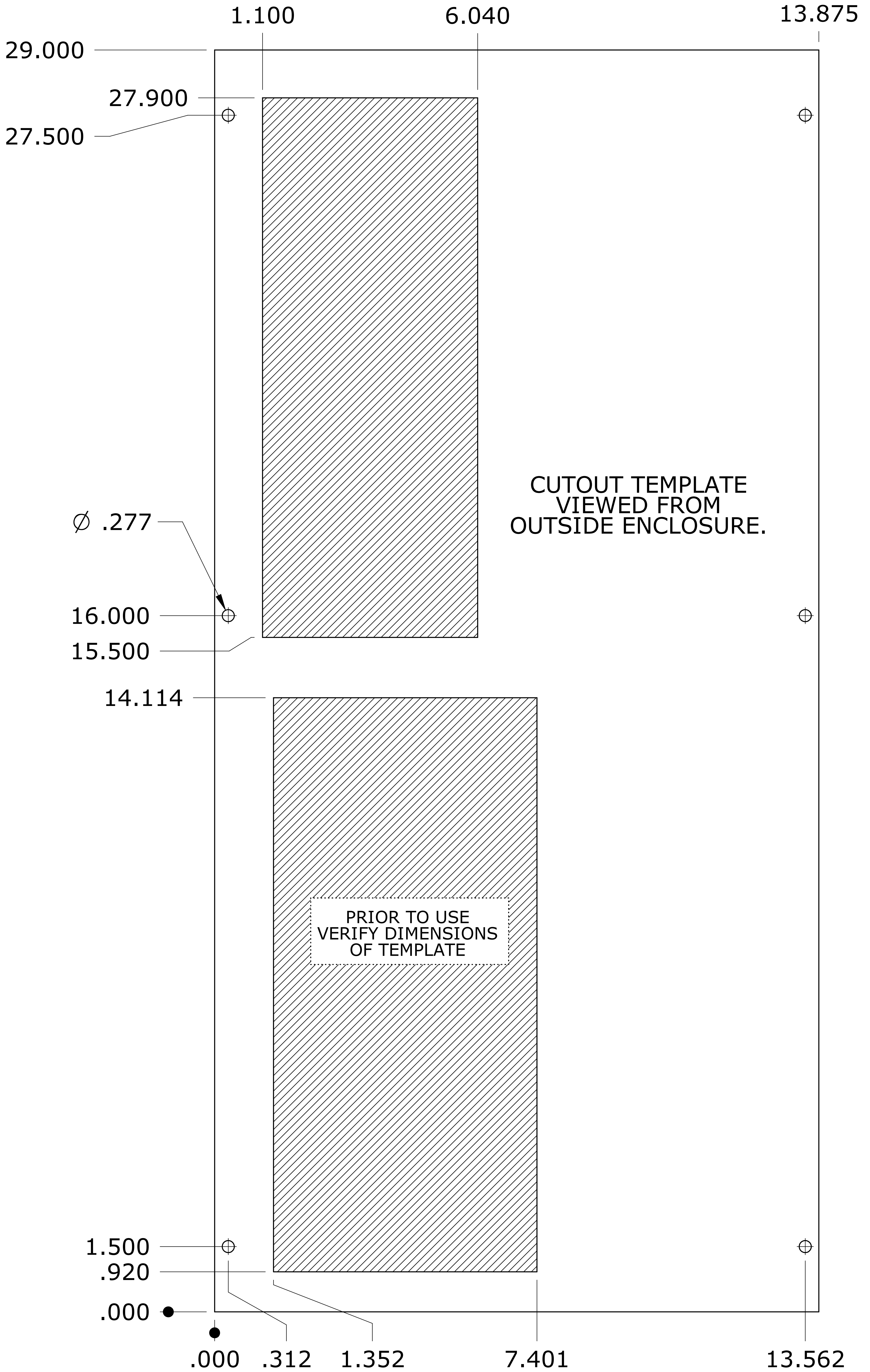
AIR TO AIR HEAT EXCHANGER A2AT_TALL CUTOUT
