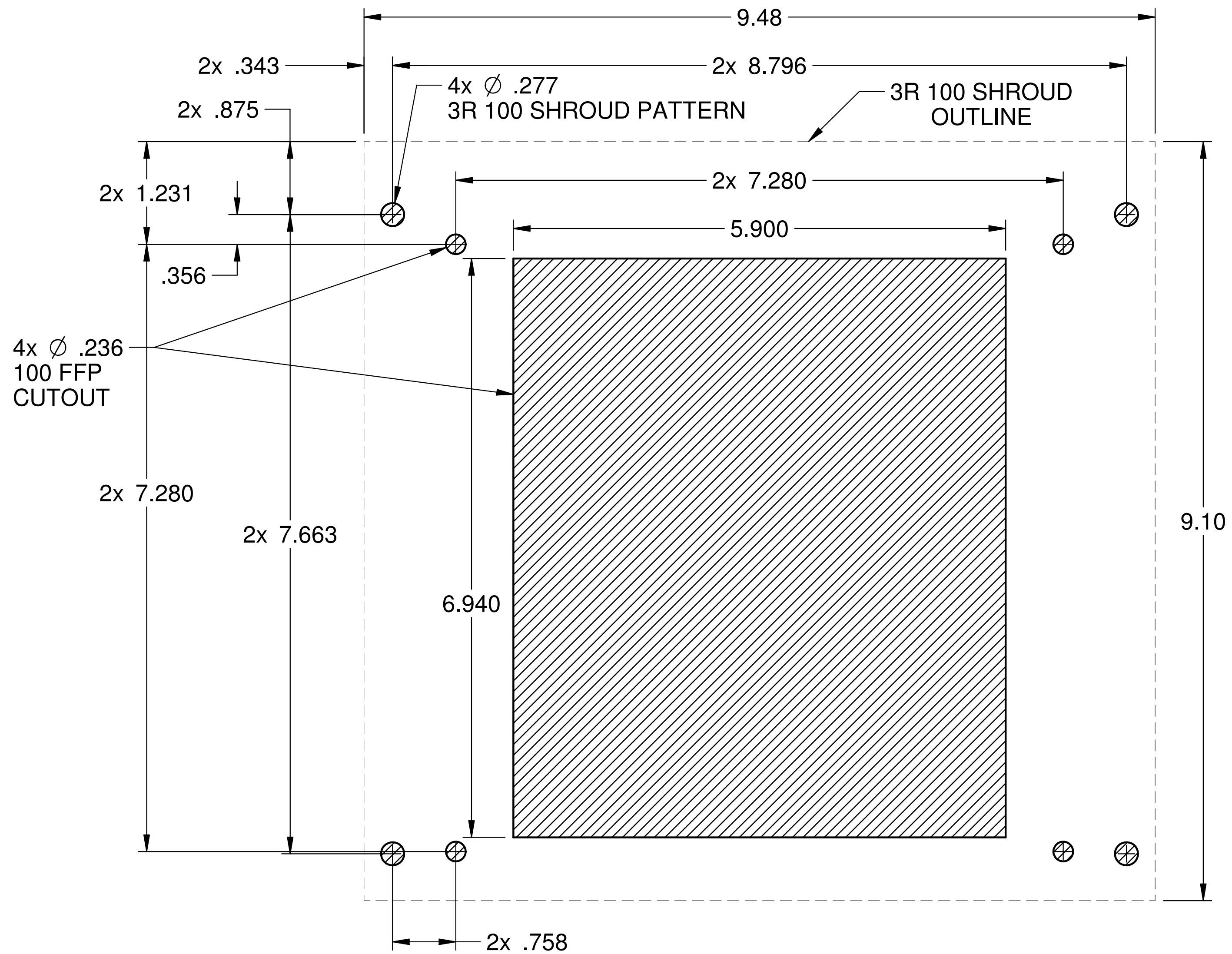
CUTOUT TEMPLATE 100 FFP WITH 3R 100 RAIN SHROUD (VERIFY PRINT ACCURACY BEFORE USE)
