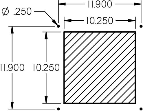
500 MFFP CUTOUT DRAWING 1:8
